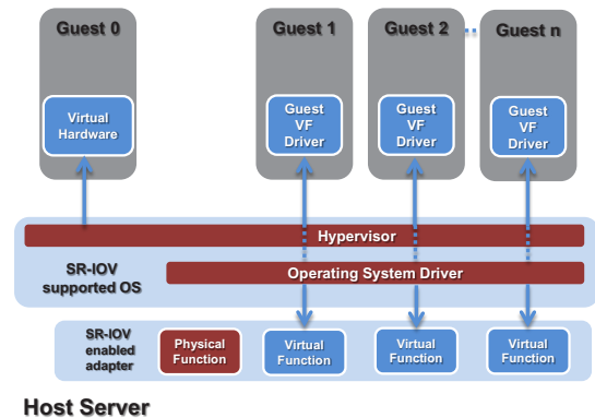
Figure 2. SR-IOV
