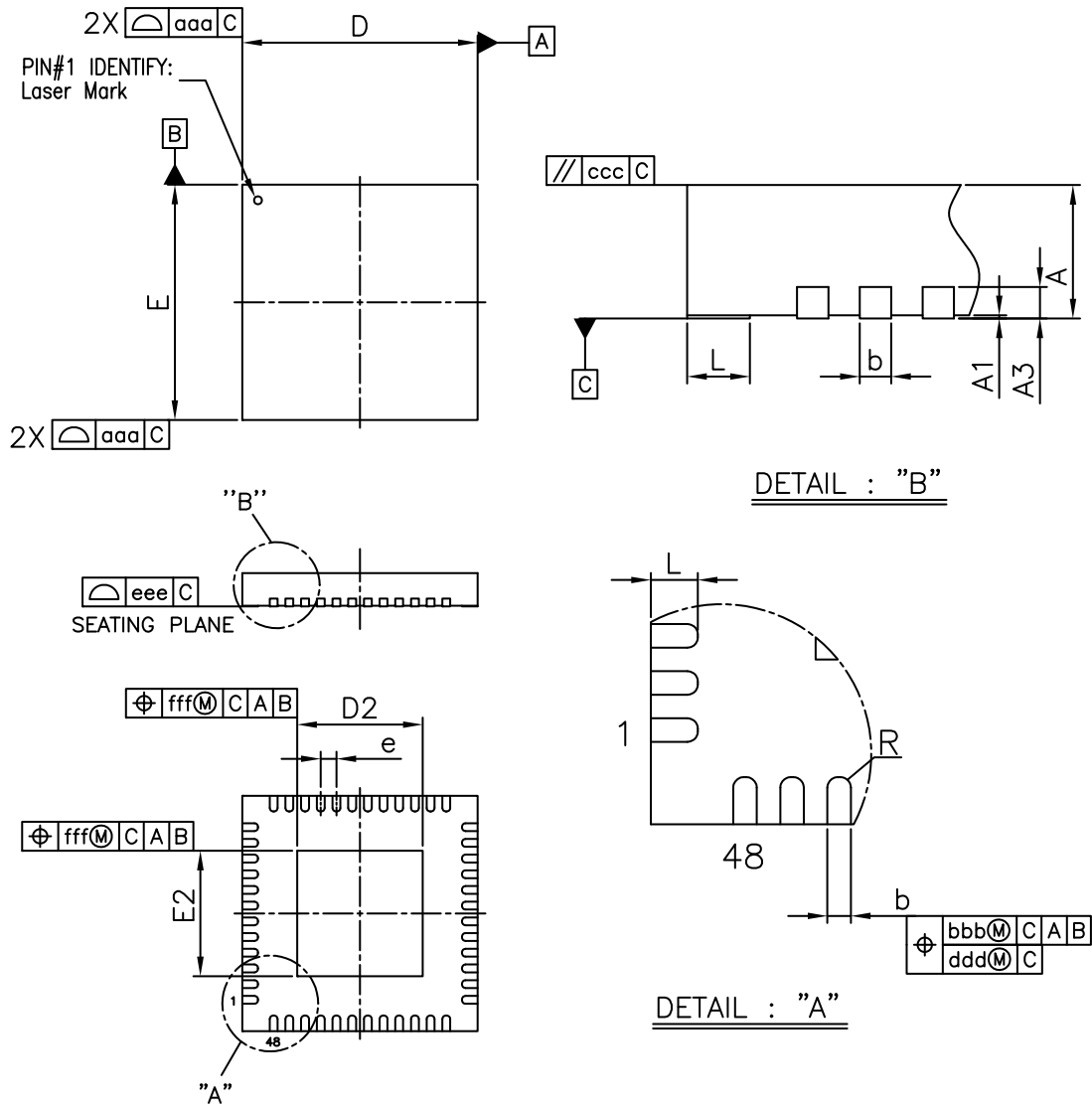
Figure 3-2 Mechanical Drawing
