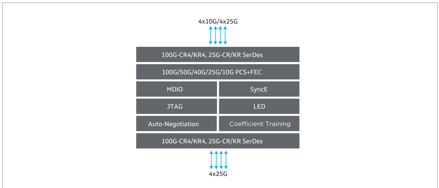
Marvell Alaska C 88X5113 Transceiver
