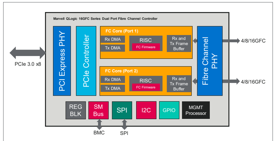
Figure 1. HPE SN1100Q Block Diagram
