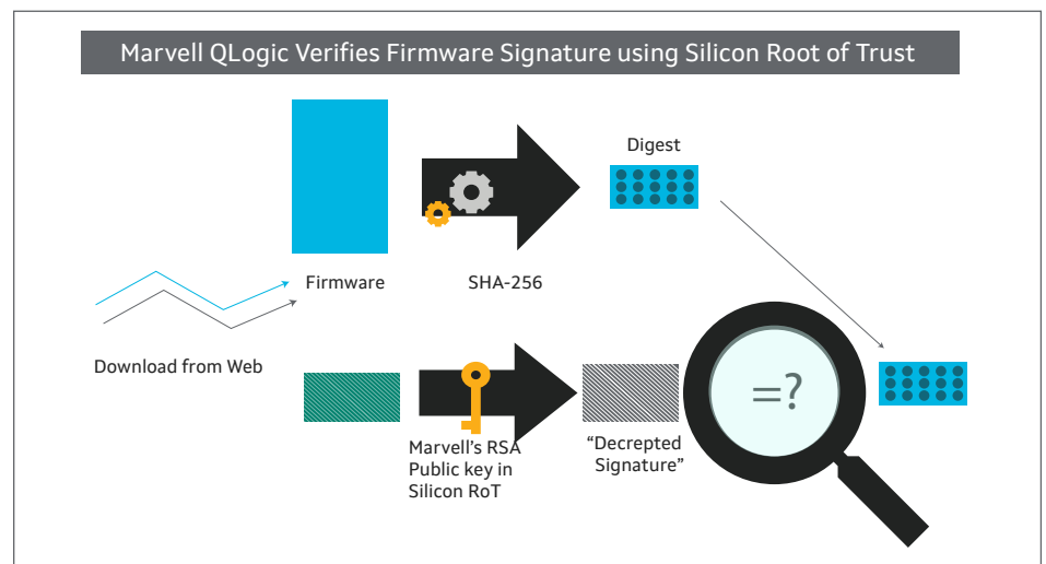
Figure 1. Marvell QLogic 2770 Series firmware verification using RSA public key
